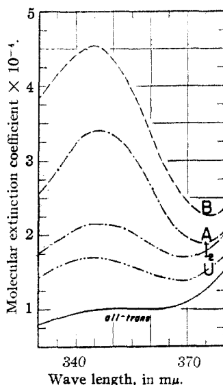
Fig. 4.—Molecular extinction curves of some members of the stereoisomeric cryptoxanthin set in the cis -peak region, in benzene. I_2 indicates the equilibrium mixture obtained upon iodine catalysis.
