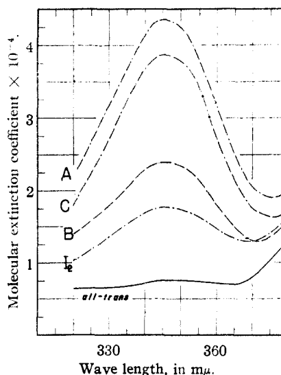
Fig. 5.—Molecular extinction curves of some members of the stereoisomeric zeaxanthin set in the cis -peak region, in benzene. I_2 indicates the equilibrium mixture obtained upon iodine catalysis.
