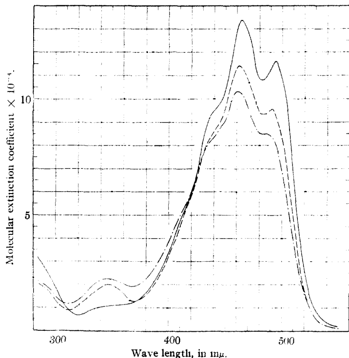
Fig. 1.—Molecular extinction curves of cryptoxanthin in benzene: —, fresh solution of the all- trans compound; ---, mixture of stereoisomers after refluxing for forty-five minutes; — · —, after iodine catalysis at room temperature in light.
