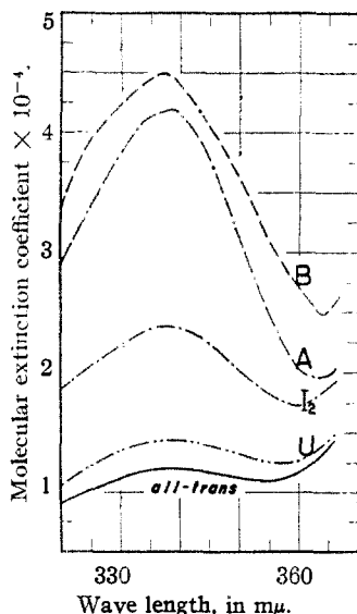
Fig. 3.—Molecular extinction curves of some members of the stereoisomeric cryptoxanthin set in the cis -peak region, in hexane. I_2 indicates the equilibrium mixture obtained upon iodine catalysis.
